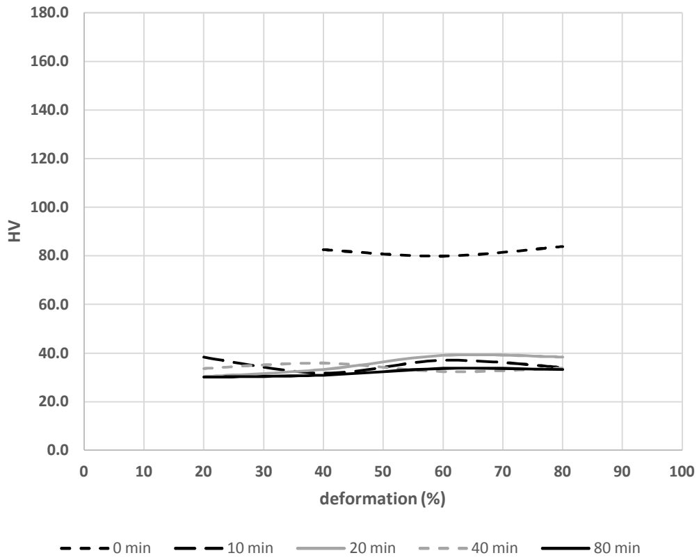
CuAs-1: HV vs. deformation (%)
