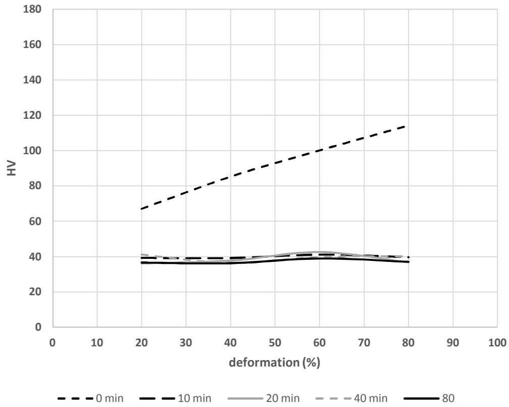
CuAs-3: HV vs. deformation (%)
